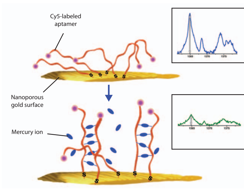
Within the sensor, mercury ions cause aptamers to bind together in pairs, pulling the cyanine 5 (Cy5) fluorescent tags away from the gold surface and therefore changing the intensity of the Raman signal (inset graphs).
